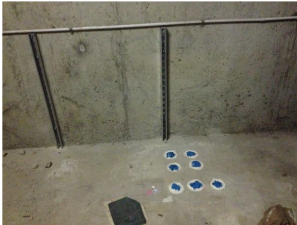
Plantroom showing cored holes with temporary firestopping and vertical Flexistrut rack to which your pipework will be clamped.
